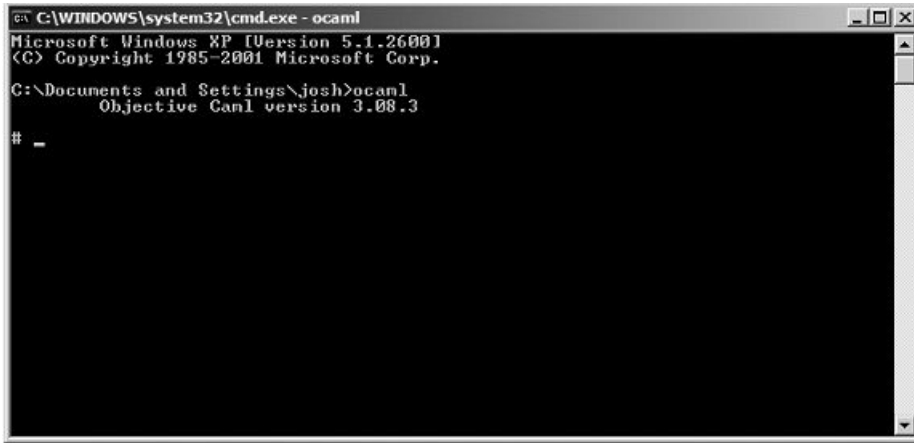
Figure 2-2. Command-line toplevel
