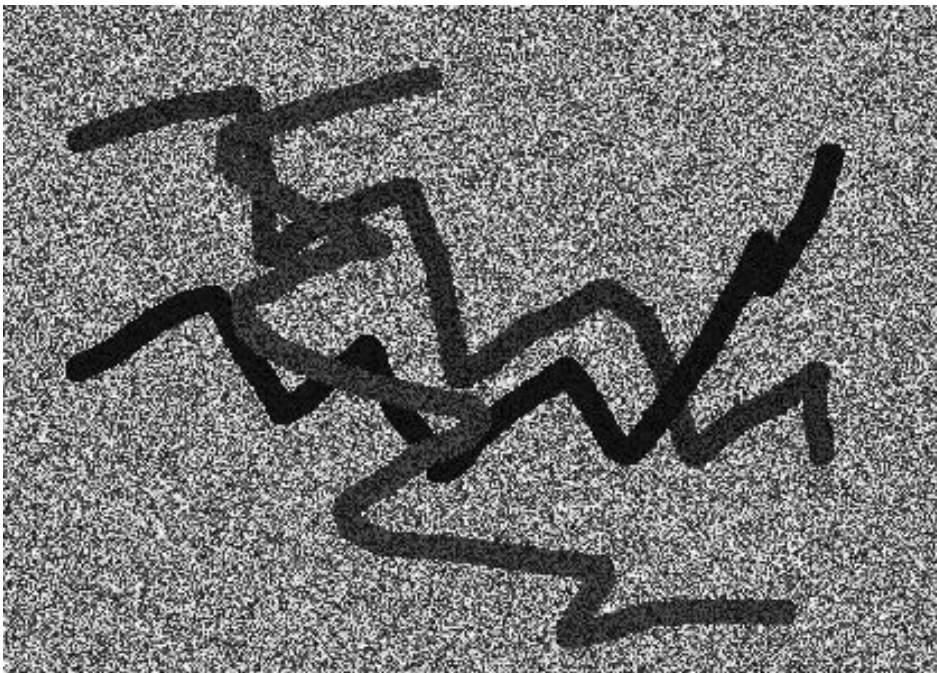
Figure 27-4. and BMP
